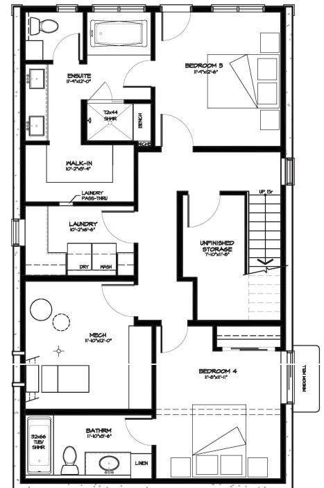
LOWER FLOOR PLAN (optional)
