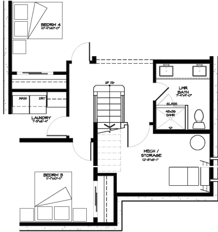
LOWER FLOOR PLAN (optional) DEVELOPED LOWER AREA: 901 SQ. FT.
