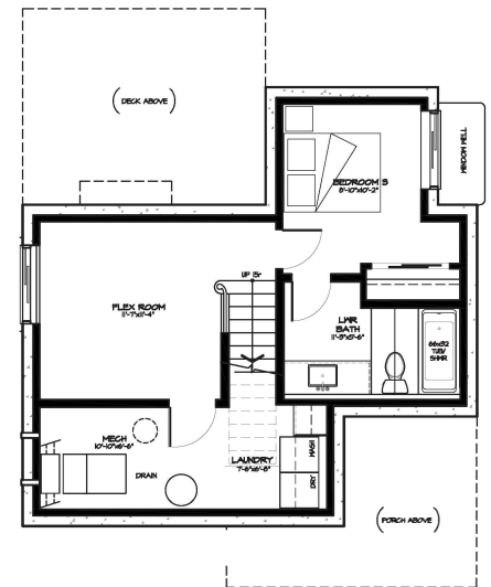
LOWER FLOOR PLAN (optional) DEVELOPED LOWER AREA: 553 SQ. FT.
