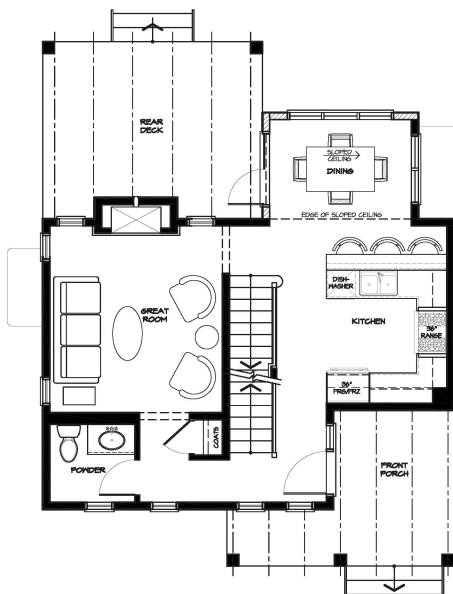
MAIN FLOOR PLAN MAIN FLOOR AREA: 621 SQ. FT.
